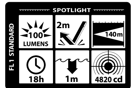
XPP-5456G SPOTLIGHT PERFORMANCE CURVE
