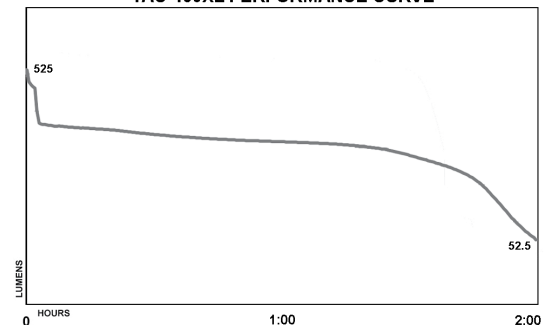
TAC-460XL PERFORMANCE CURVE
