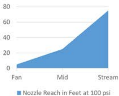
Nozzle Reach in Feet at 100 psi
